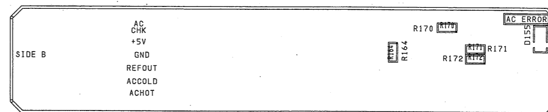
TU-RECT SUB (PT-1607C) (PHASE II) SIDE B
