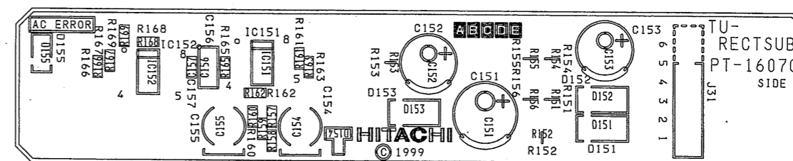
TU-RECT SUB (PT-1607C) (PHASE II) SIDE A
