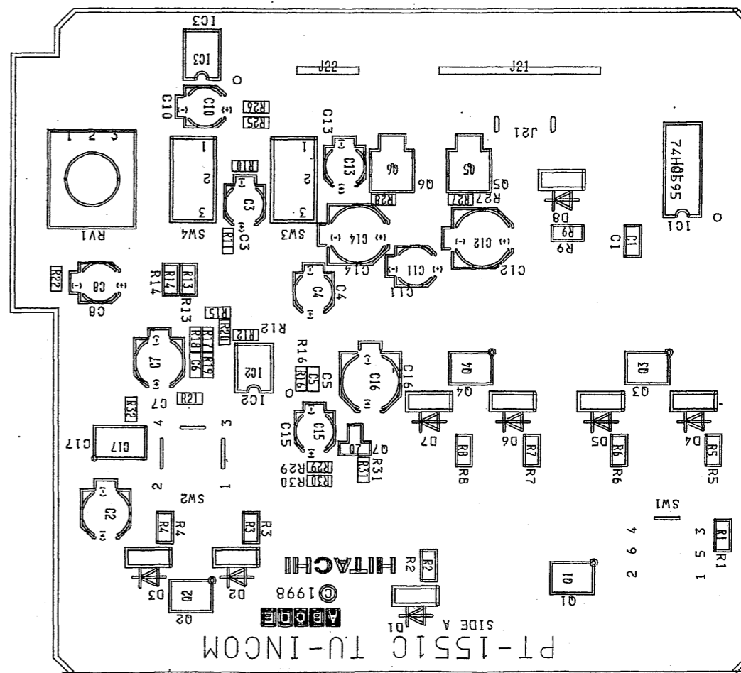
INCOM/LED (PT-1551C) SIDE B
