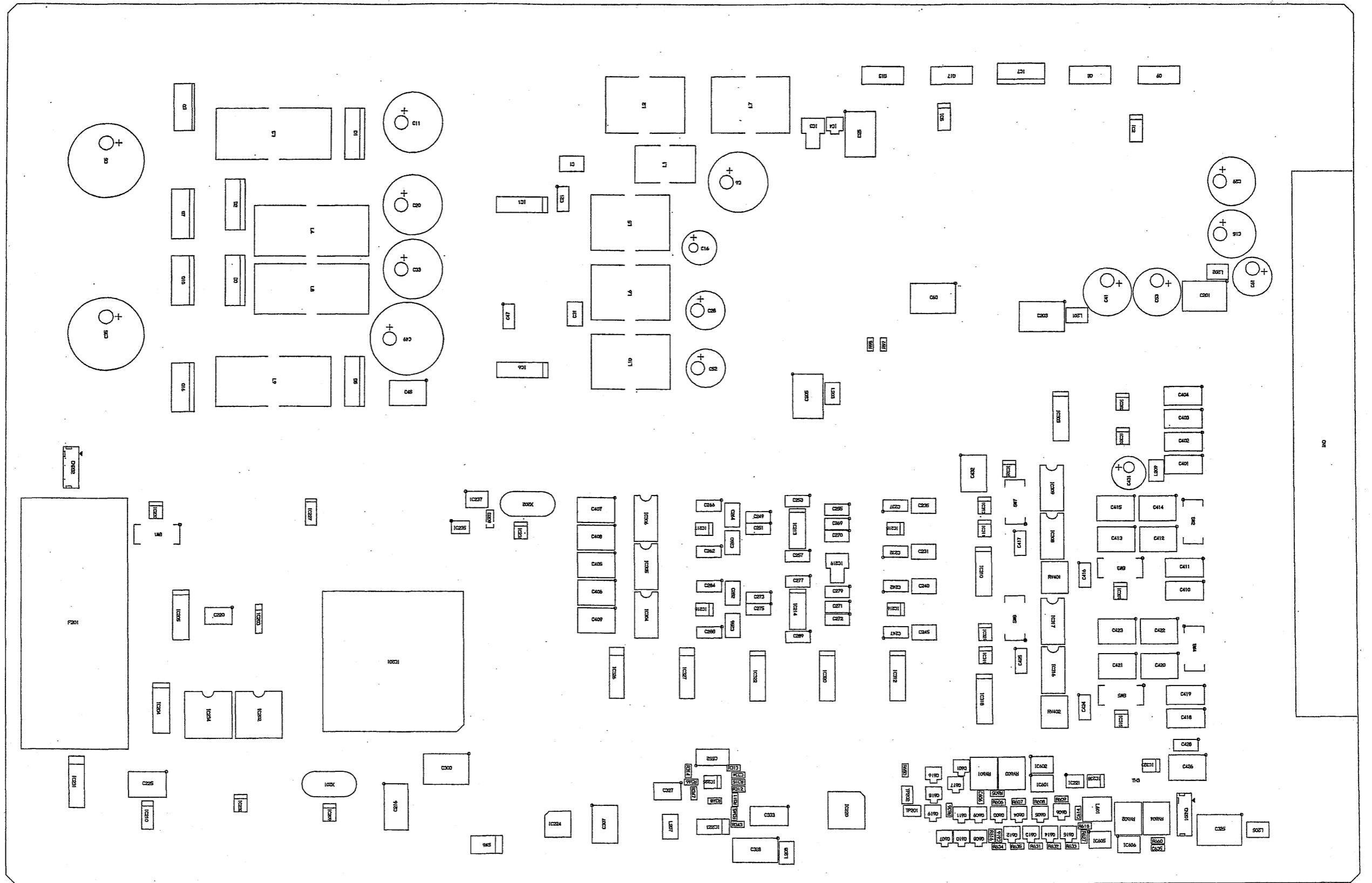
TU-POWER/INCOM(PT-1519D) SIDE A
